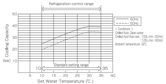
Graph of Cooling Capacity with Cooling Unit
