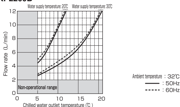
RKP2200B
