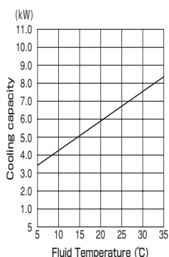
RKE1500B1-VW-G1·G2
